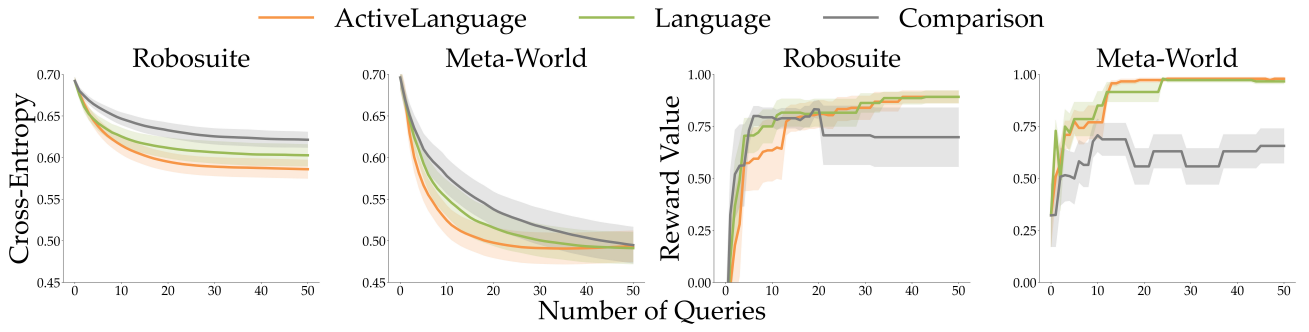
Figure 6. Reward learning evaluation in cross-entropy and reward value results for test set queries are shown for the ACTIVELANGUAGE, LANGUAGE, and COMPARISON methods in the Robosuite and Meta-World environments (mean \pm s.e. over 5 seeds). The usage of comparative language feedback and an active query generation method triumphs over preference comparisons, as seen in both cross-entropy and reward value metrics.
